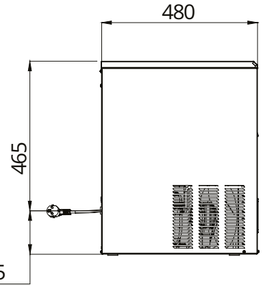
Lateral View
