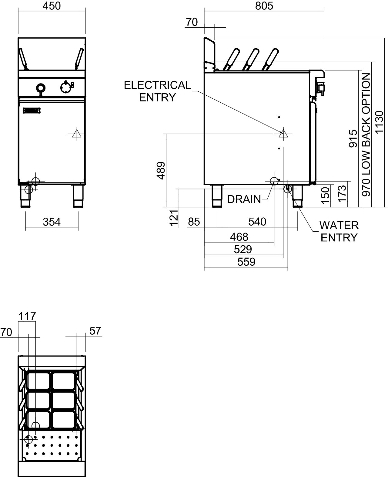
PC(1)8140E-Pasta Cooker
