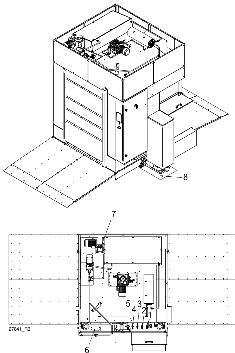
The machine installed "on the floor"
