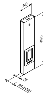
Electrical box
