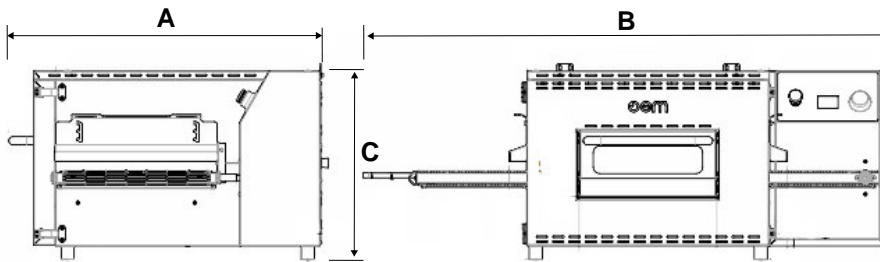
TUNNEL TVL80
